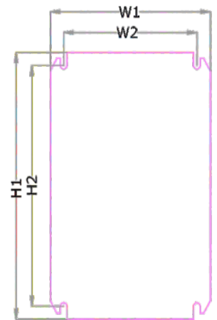
MOUNTING PLATE GI - 2.0mm
